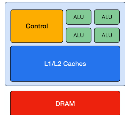
Figure 5.1: Simplified CPU [4]
